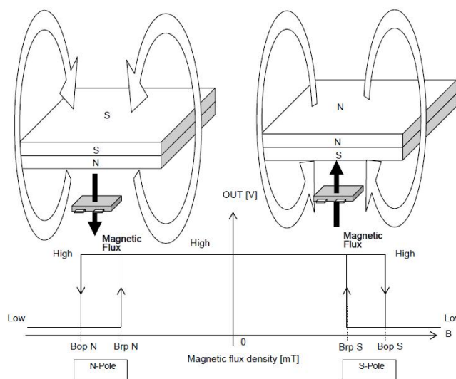
Figure 3, Magnetic Operation Characteristic of AS1829A
