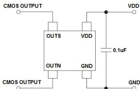
Figure 1, Typical Application Circuit of AS1829A
